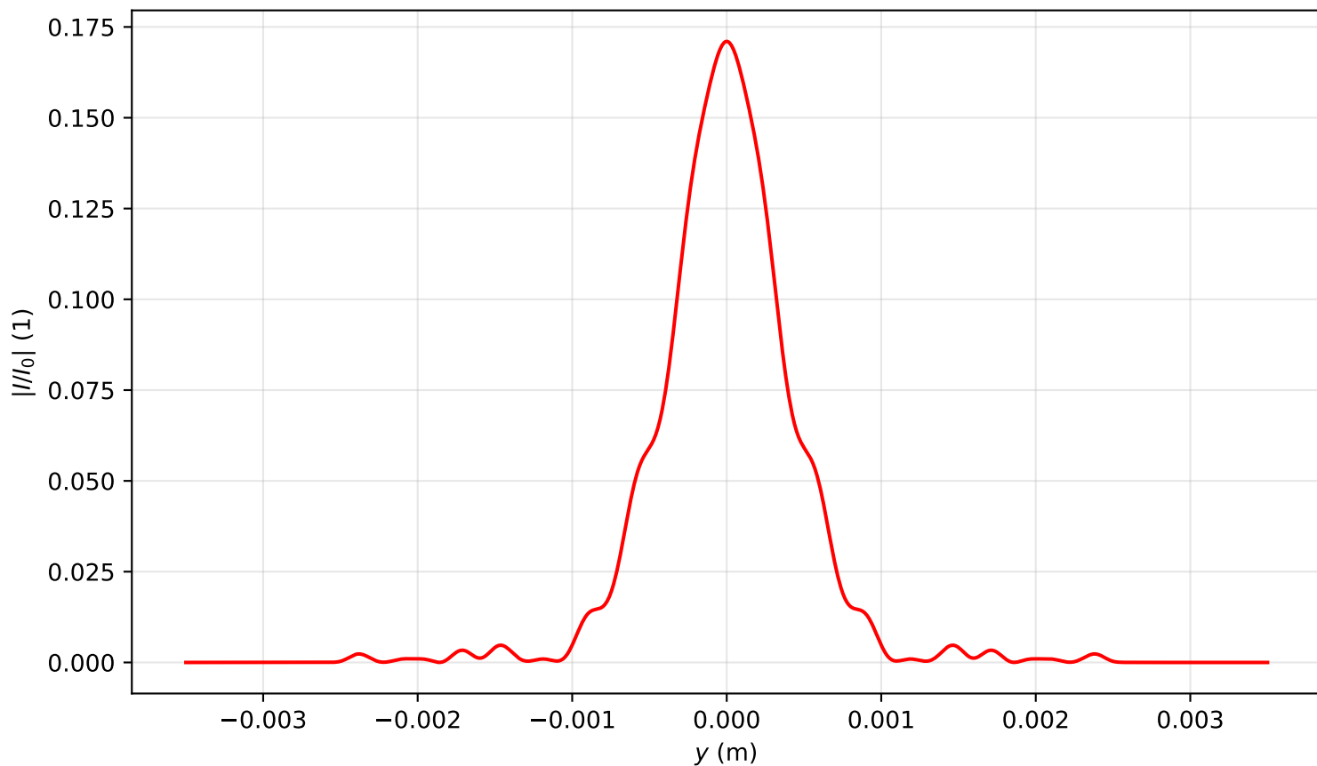
Intensity profile I(x=0, y, z=2.388)/I_0 , \text{Pin}=5.0\text{Pcr} , artificial time
